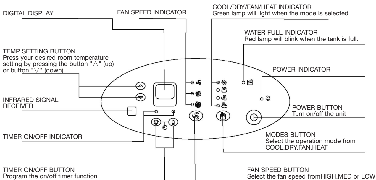
Operating panel
